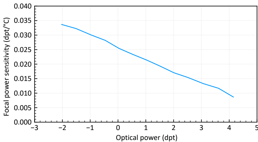
Figure 11: Temperature sensitivity as a function of focal power.
