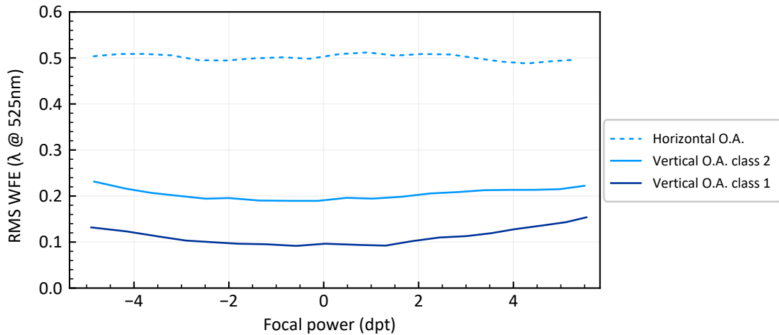
Figure 8: Typical wavefront error of the EL-16-40-TC vs focal power with optical axis vertical and horizontal (@525nm, measured over 80% of the clear aperture, defocus, tilt and sphere excluded).
