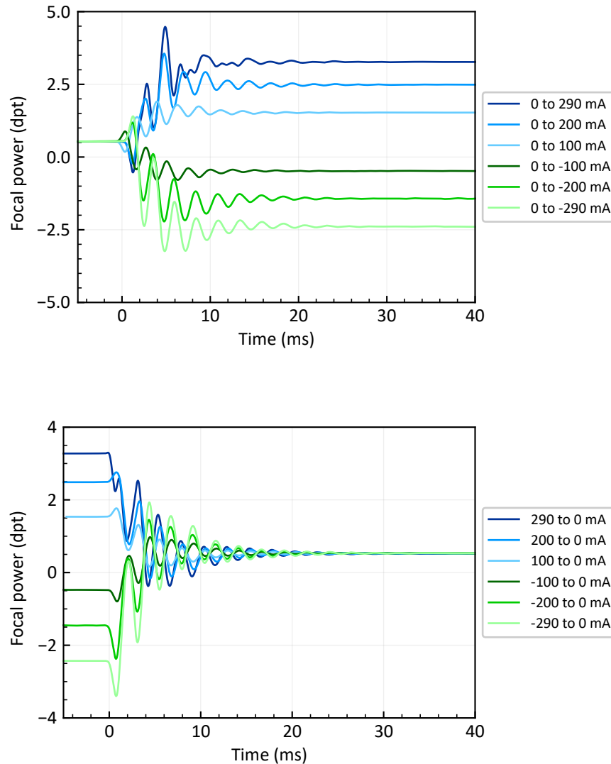
Figure 9: Typical optical response of the EL-16-40-TC-VIS-5D for several current steps. The upper plot shows a series of steps from low to high current and the lower plot for steps from high to low current.
