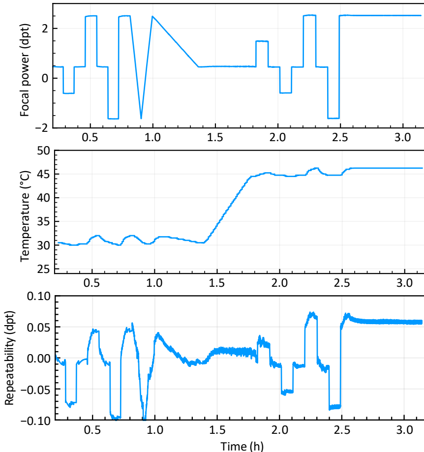
Figure 12: Repeatability measurement over a time span of about 3 hours. Optical power and environmental temperature are varied over a broad range while the error between measured and set optical power remains small.
