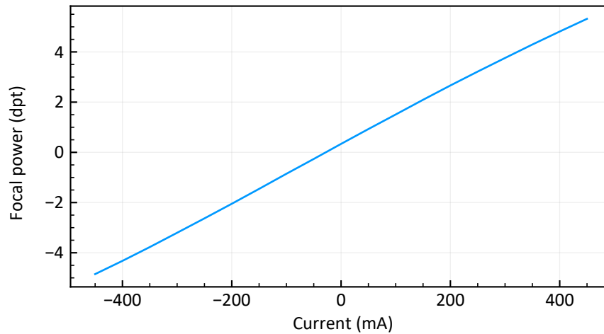
Figure 6: Typical data showing the relation between focal power (in diopters) and electrical current.
