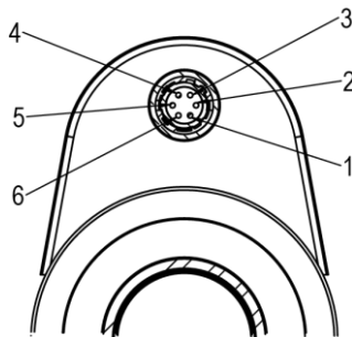
Figure 5: Electrical connections of the Hirose connector. The pinout is the same for all adapter versions.
